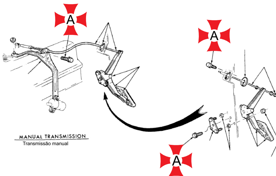
ACCELERATOR LINKAGE 1973/77 MAVERICK--6 CYL.
