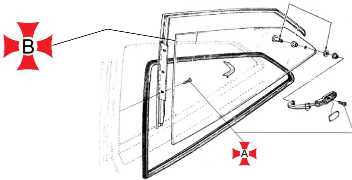
QUARTER WINDOW and RELATED PARTS 1973/77 MAVERICK-BODY
