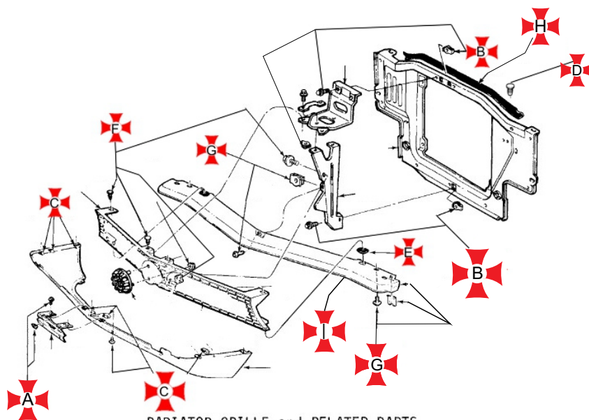
RADIATOR GRILLE and RELATED PARTS 1973 MAVERICK
