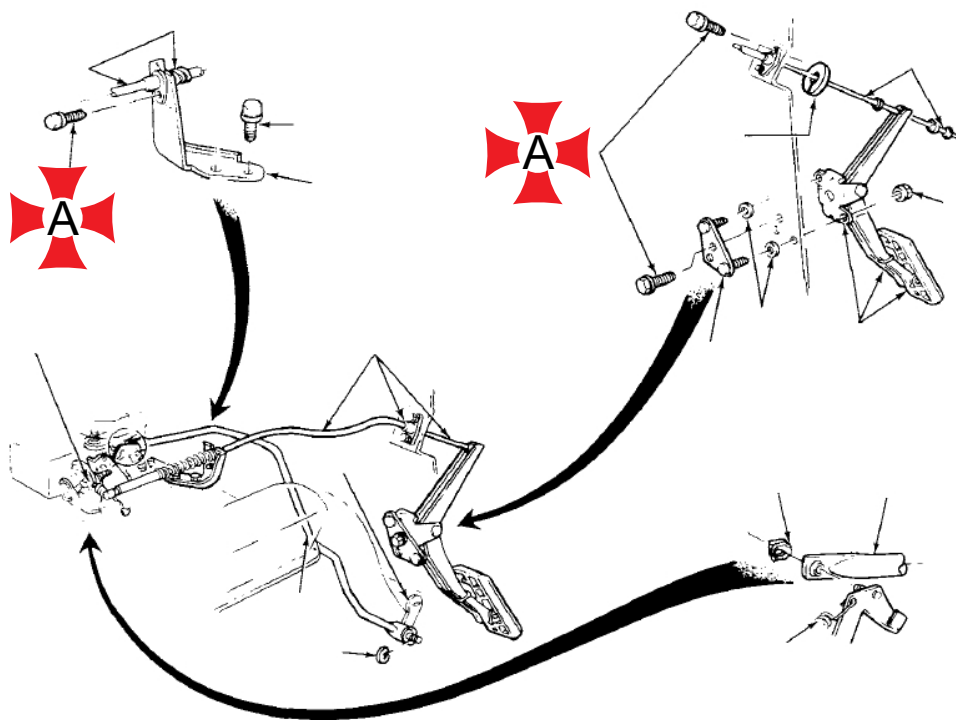
ACCELERATOR LINKAGE MAVERICK--8 CYL. 1975/76
