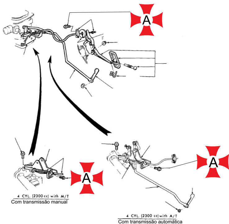
ACCELERATOR LINKAGE 1974/77 MAVERICK 4 CYL. (2300 cc)
