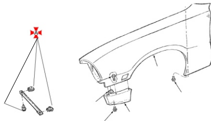
FENDERS and RELATED PARTS 1974/77 MAVERICK
