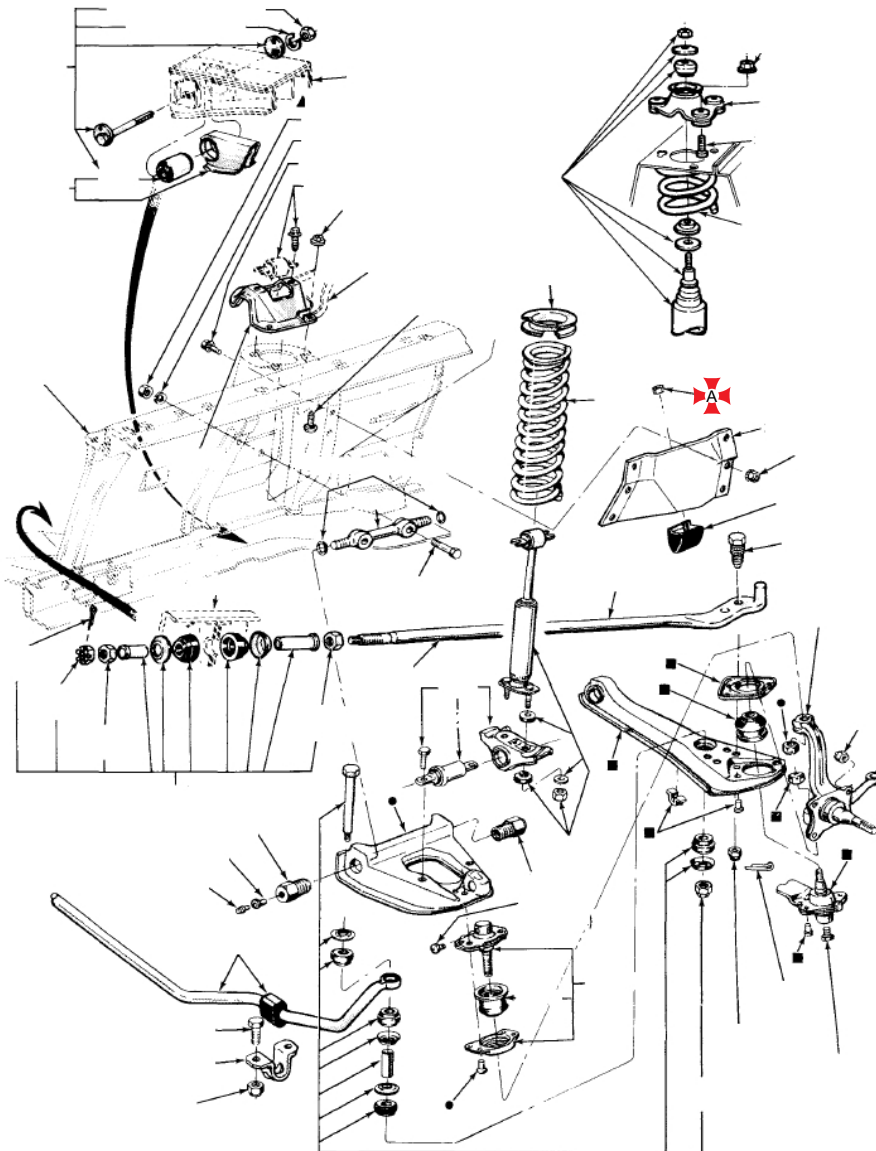
FRONT SUSPENSION 1973/77 MAVERICK
