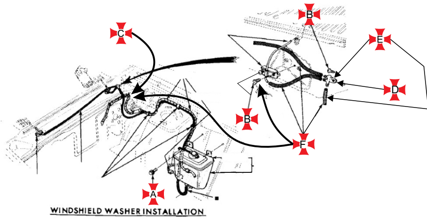
WINDSHIELD WIPER and WASHER 1973/77 MAVERICK
